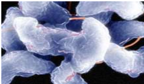
Campylobacter bacteria http://www.biocontrolsys.com/products/targets/pathogens/
